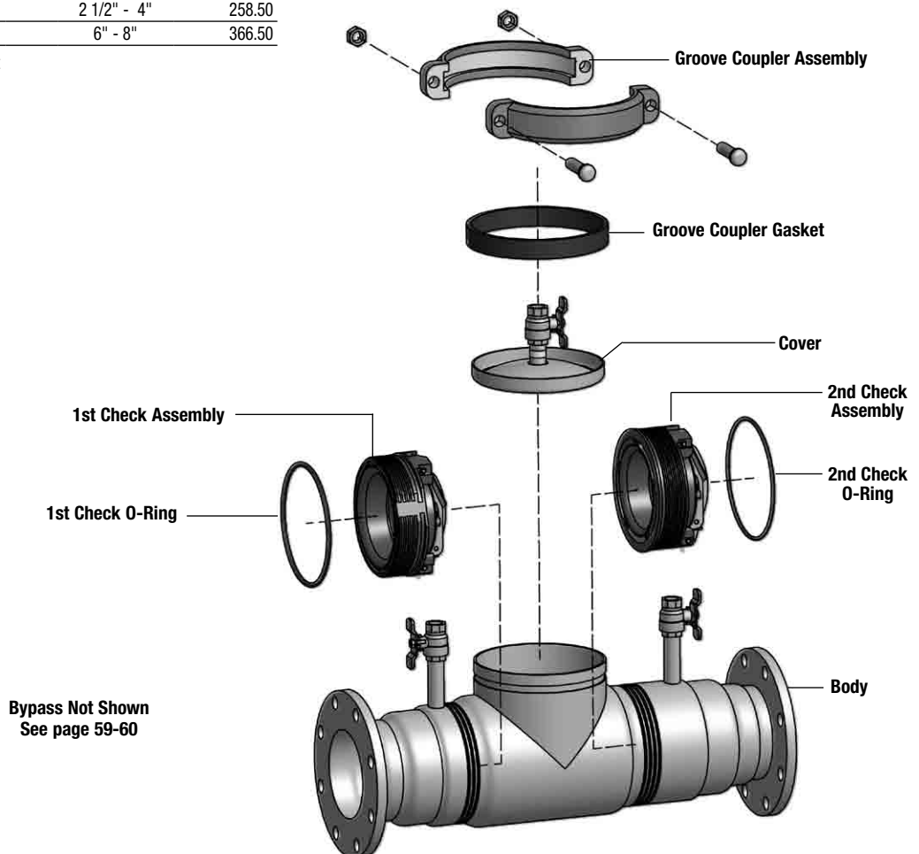
3" – 8" 2001SS/3001SS
